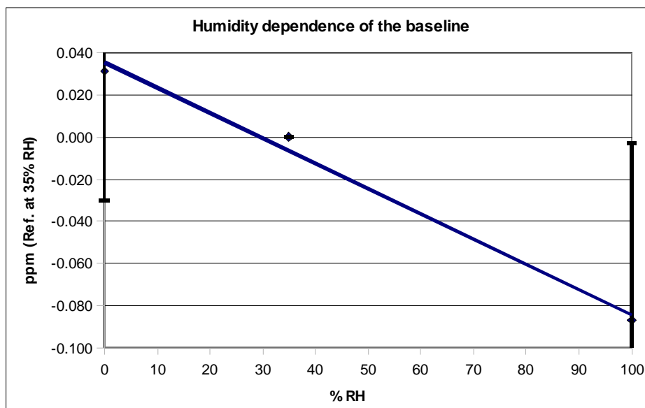
Figure 1: Humidity dependence
