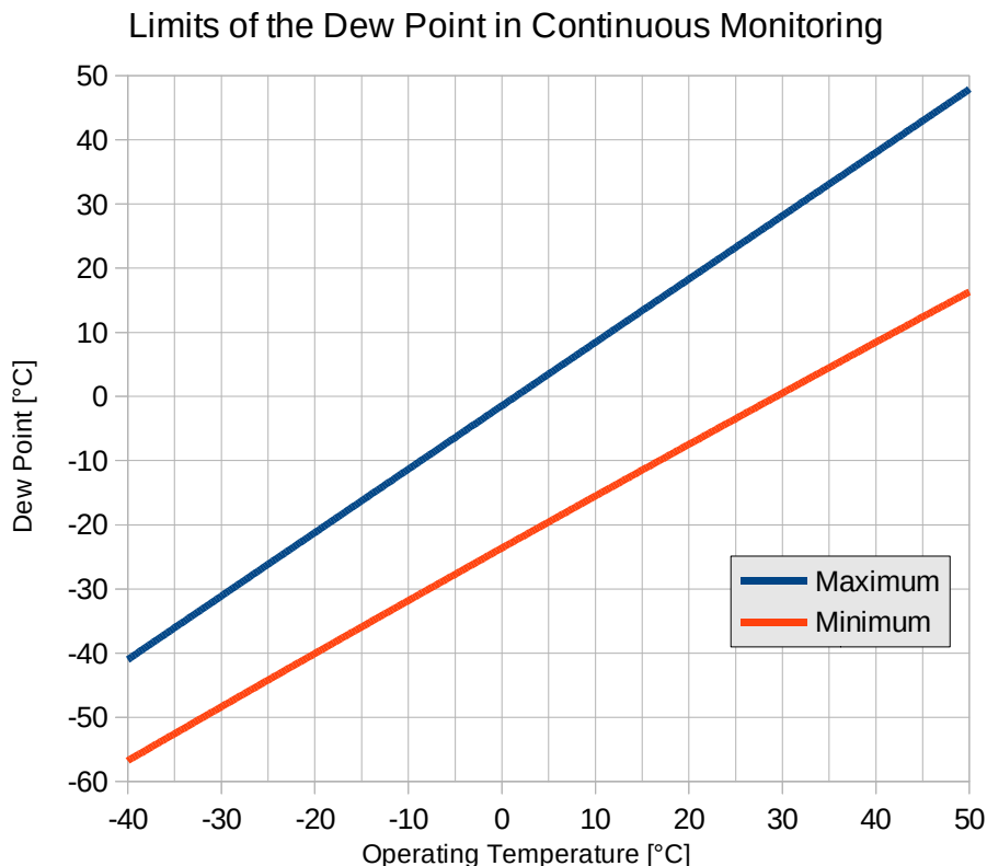
Figure 6 Allowed humidity range expressed as limits of the dew point of the gas sample Monitoring under complete dry or humid conditions can be realized with an ambient air purge cycle.
